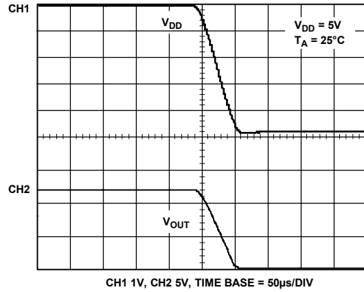
Figure 17. V DD vs. V OUT
